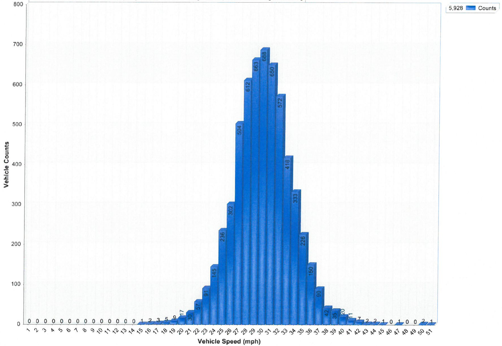
Vehicle Counts Vs. Speed [Old Springs Road- 10-14 through 10-18, 2016: Incoming Direction]
